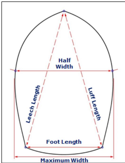
Symmetric Spinnaker
