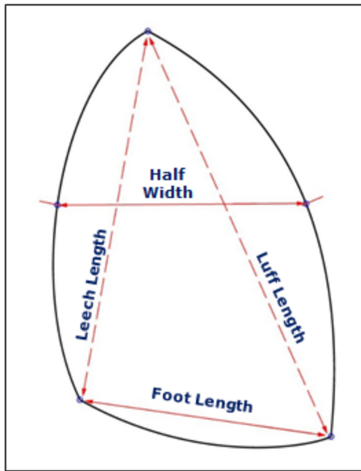
Asymmetric Spinnaker
