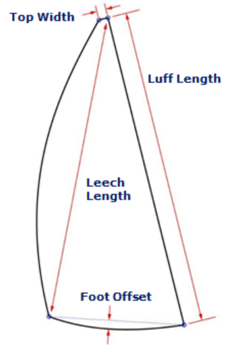
Headsail
