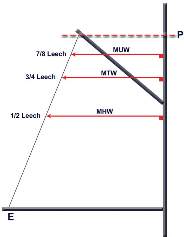
MAINSAIL WIDTHS - No Topsail
