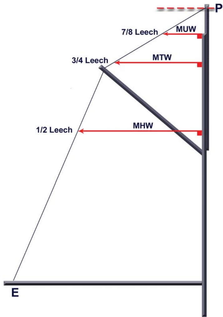
MAINSAIL WIDTHS - With Topsail
